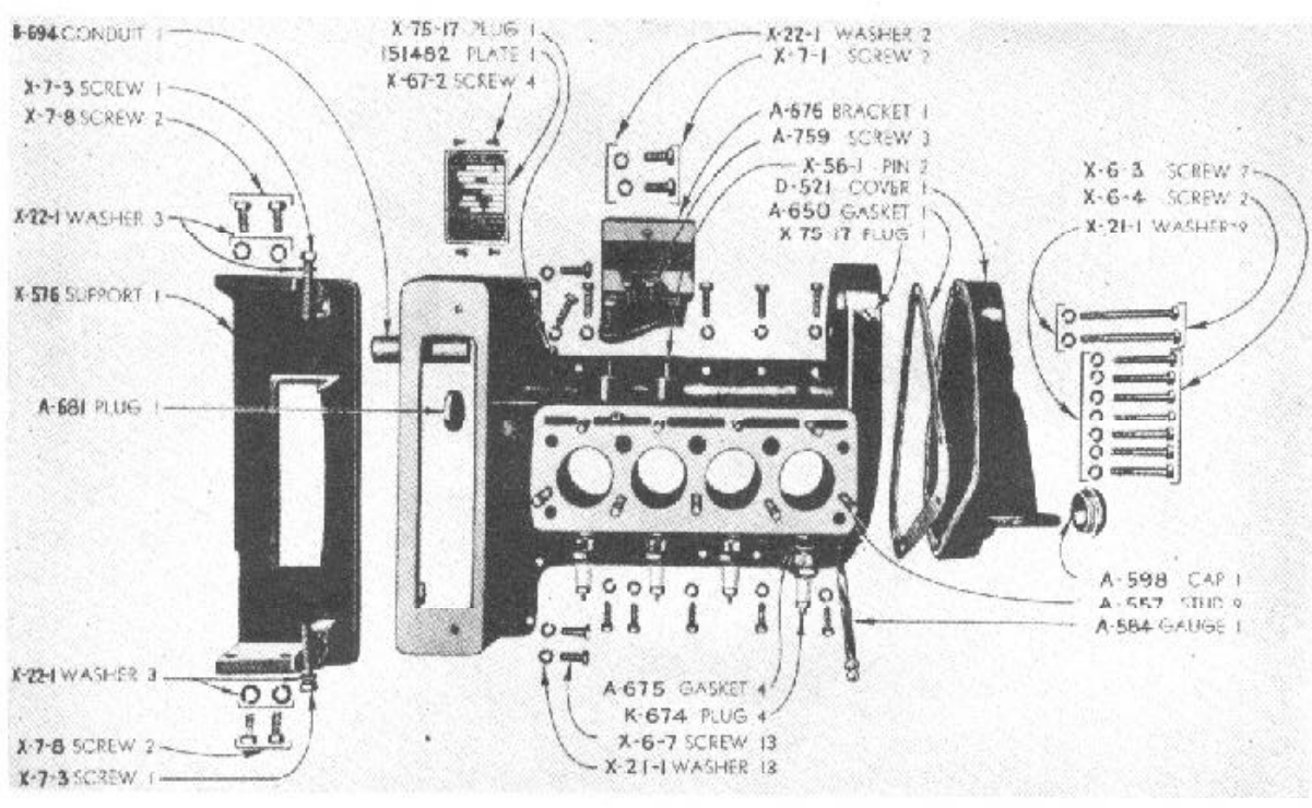
Figure 43. Cylinder block assembly.
