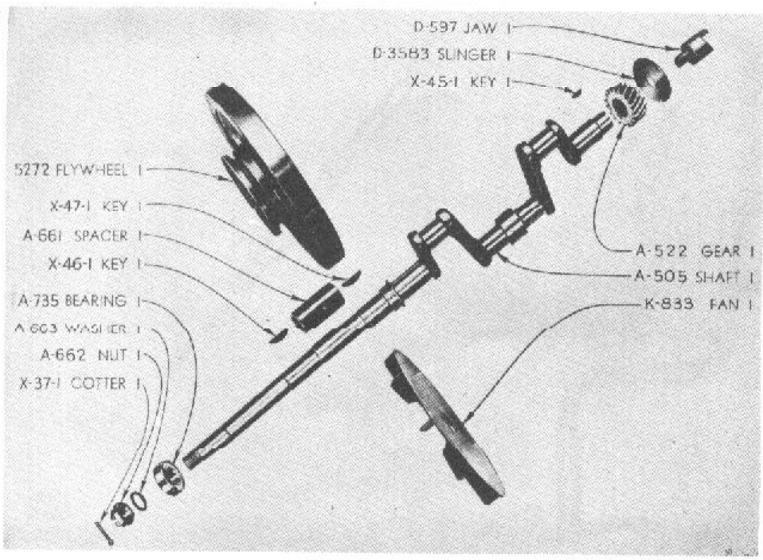
Figure 44. Crankshaft assembly.
