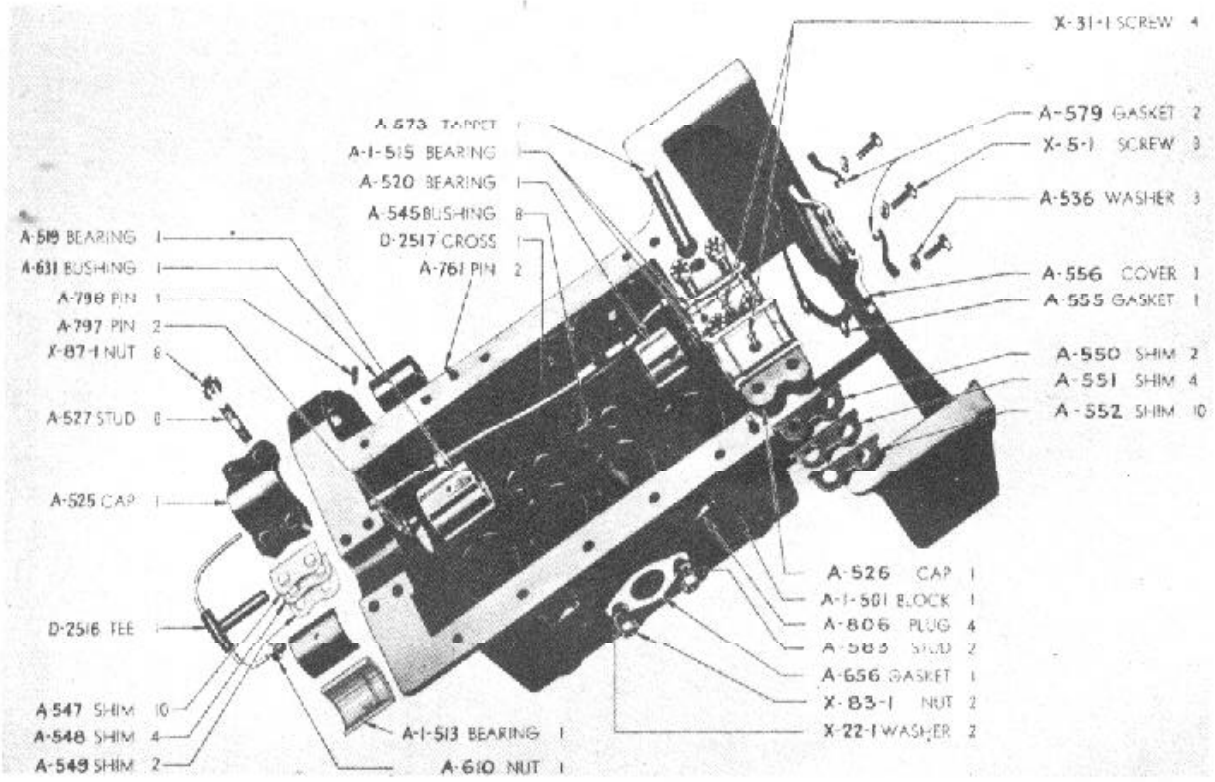
Figure 42. Cylinder block assembly.
