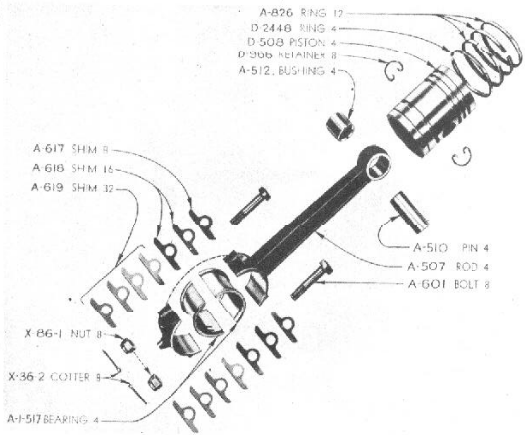
Figure 41. Piston and connecting rod assembly.
