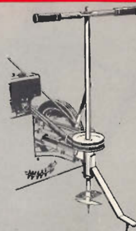
#2023 — 7" POST HOLE AUGER Drills 2' deep hole in one minute. Front end operation by one man.
