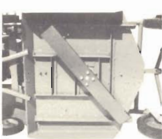
Shows 24" Bar Blade — suction type — of heat treated spring steel — holds sharp edge.
