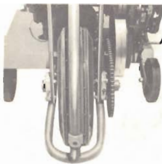
Shows final chain drive to puncture proof 16.00 x 4.00 drive tire and wheel. Also, shows tandem safety wheels.
