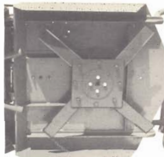
Also available, safety hinged 4 swing-blades assembly for extremely rough mowing.
